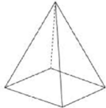
Rectangular pyramid
