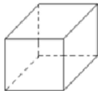
Rectangular prism
